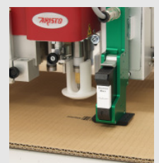
Printhead
